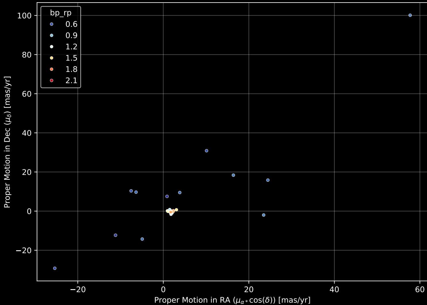
APOGEE DR17 Field: [LMC32] Proper Motion Diagram (n= 116)
