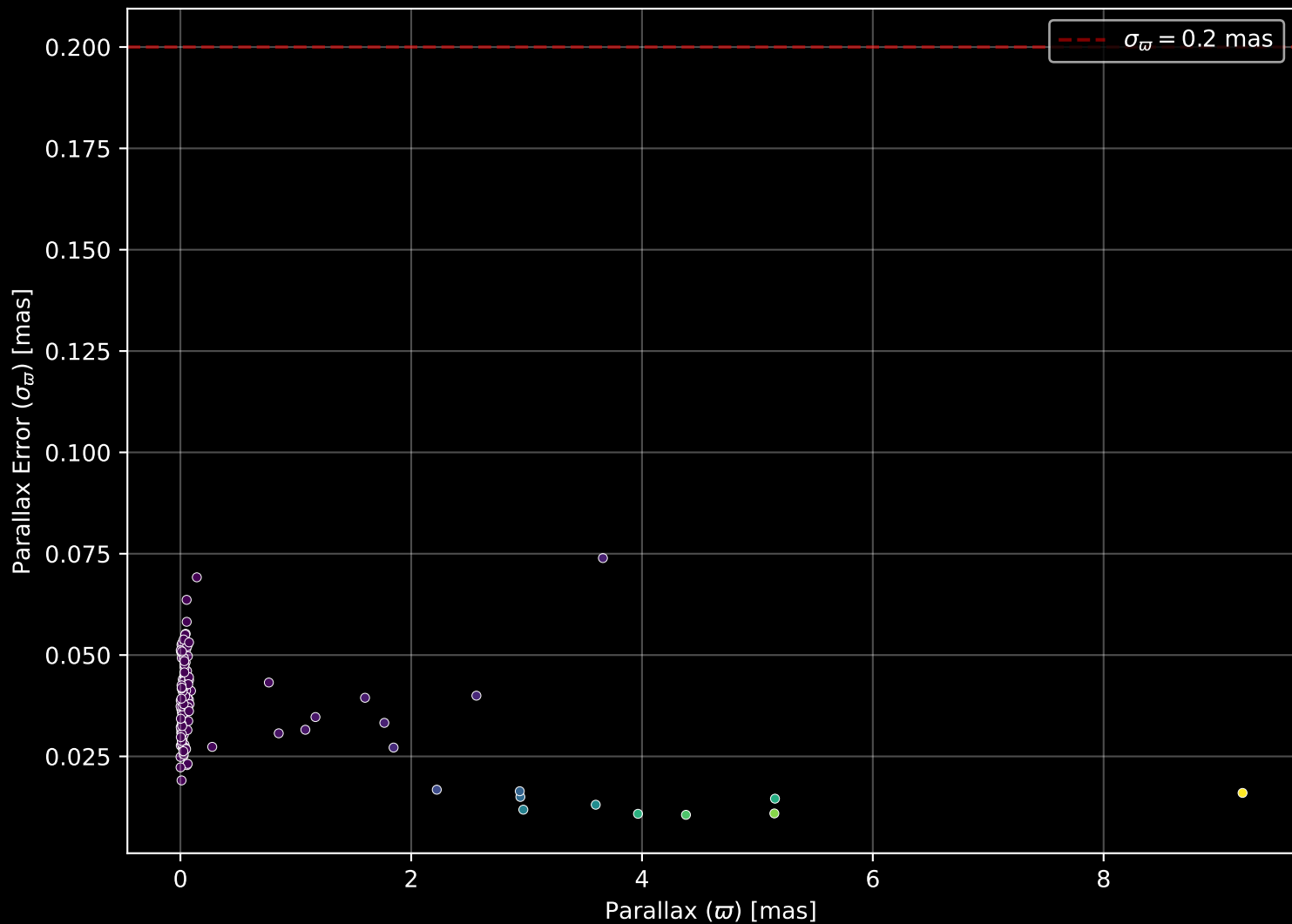
APOGEE DR17 Field: [LMC32] Parallax Quality (n= 116)
