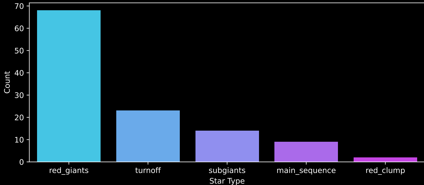
APOGEE DR17 Field: [LMC32] Count plot of Star Type
