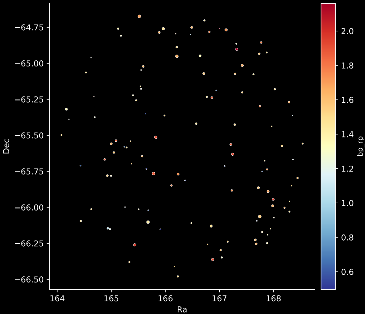
APOGEE DR17 Field: [LMC32] Stars: 116
