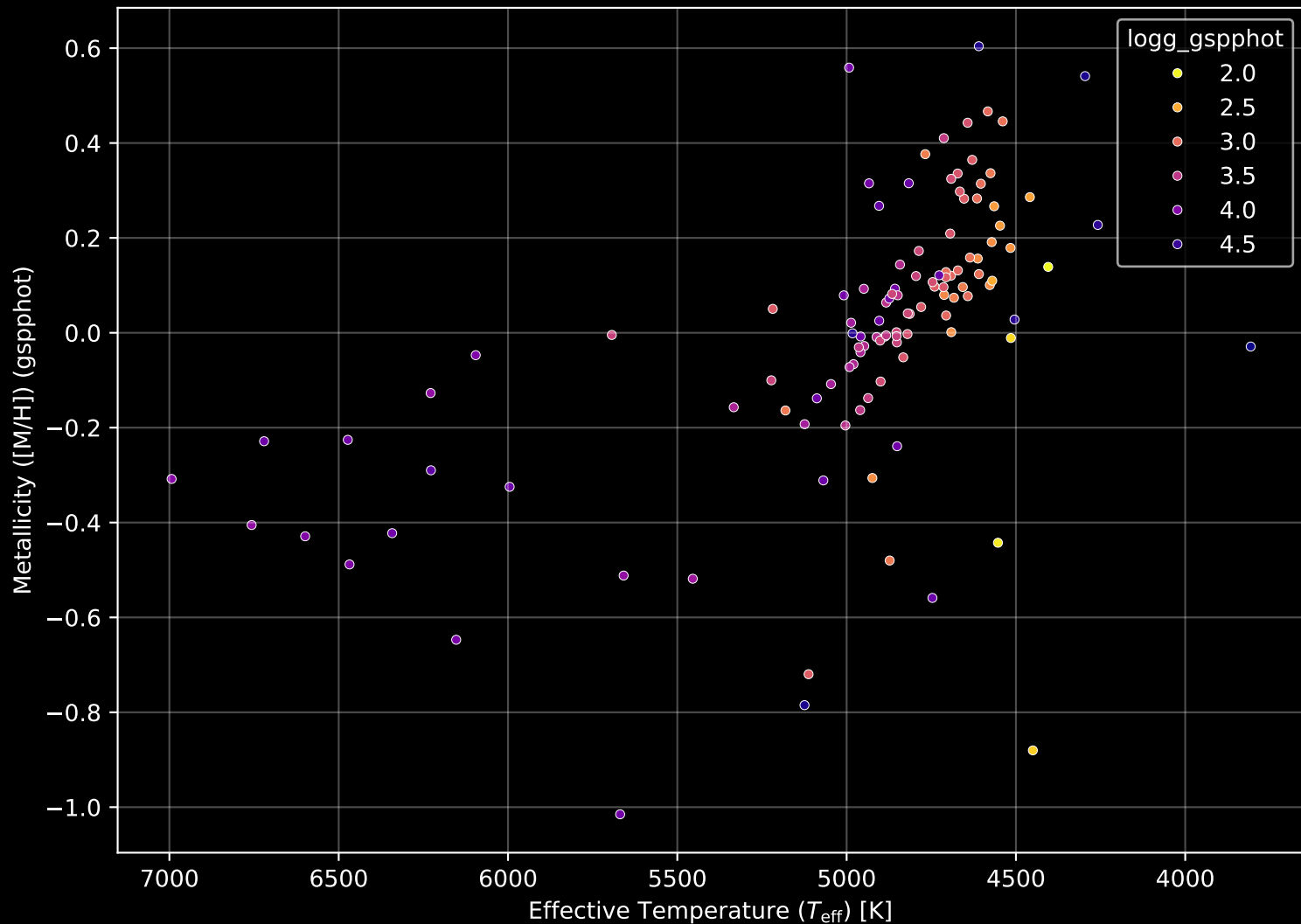
APOGEE DR17 Field: [LMC32] Stellar Population Parameters (n= 116)
