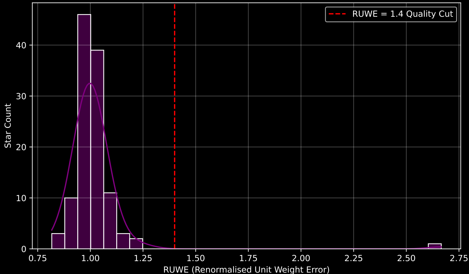
GAPOGEE DR17 Field [LMC32] RUWE Distribution (n= 115)
