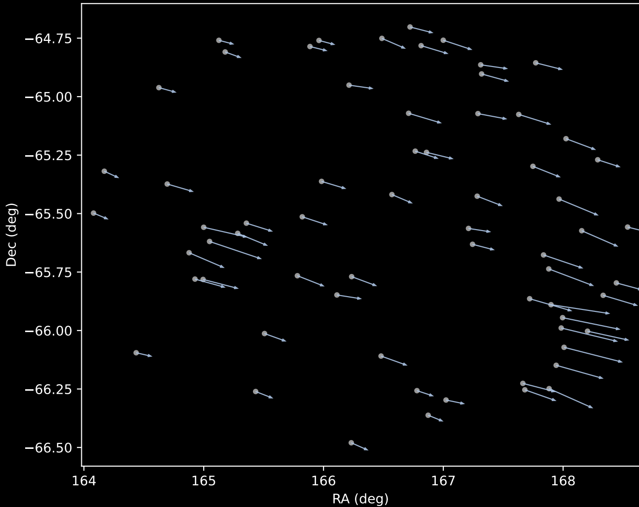
APOGEE DR17 Cluster 1 Proper Motion Vectors (n=65)
