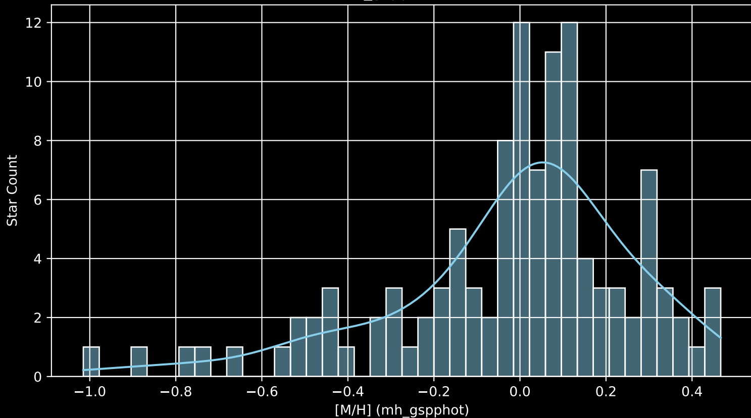
APOGEE DR17 Field: [LMC32 [M/H] (mh_gspphot) (n= 113)
